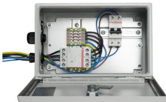
Control box (230V / 3*400V + N)
